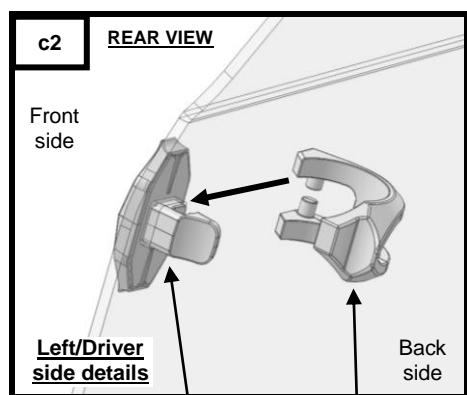
TRR windshield hook TRR cage clamp
